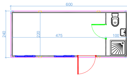
CON-25
